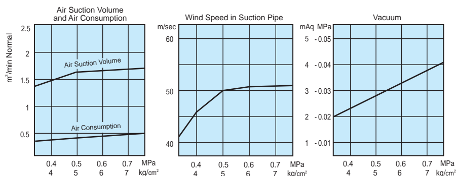
■ Performance Chart ( SC30-32S, SC20-32, SC20-32P )
